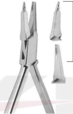
AKI 3202 Adams Tweed loop forming pliers. For forming loop in wires up to 0,56 mm. (.22").
